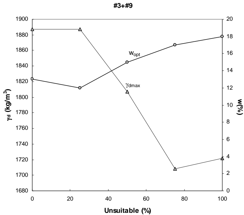
Figure 5(d). Dry density vs. moisture content for mixture of soils 9 and 3
