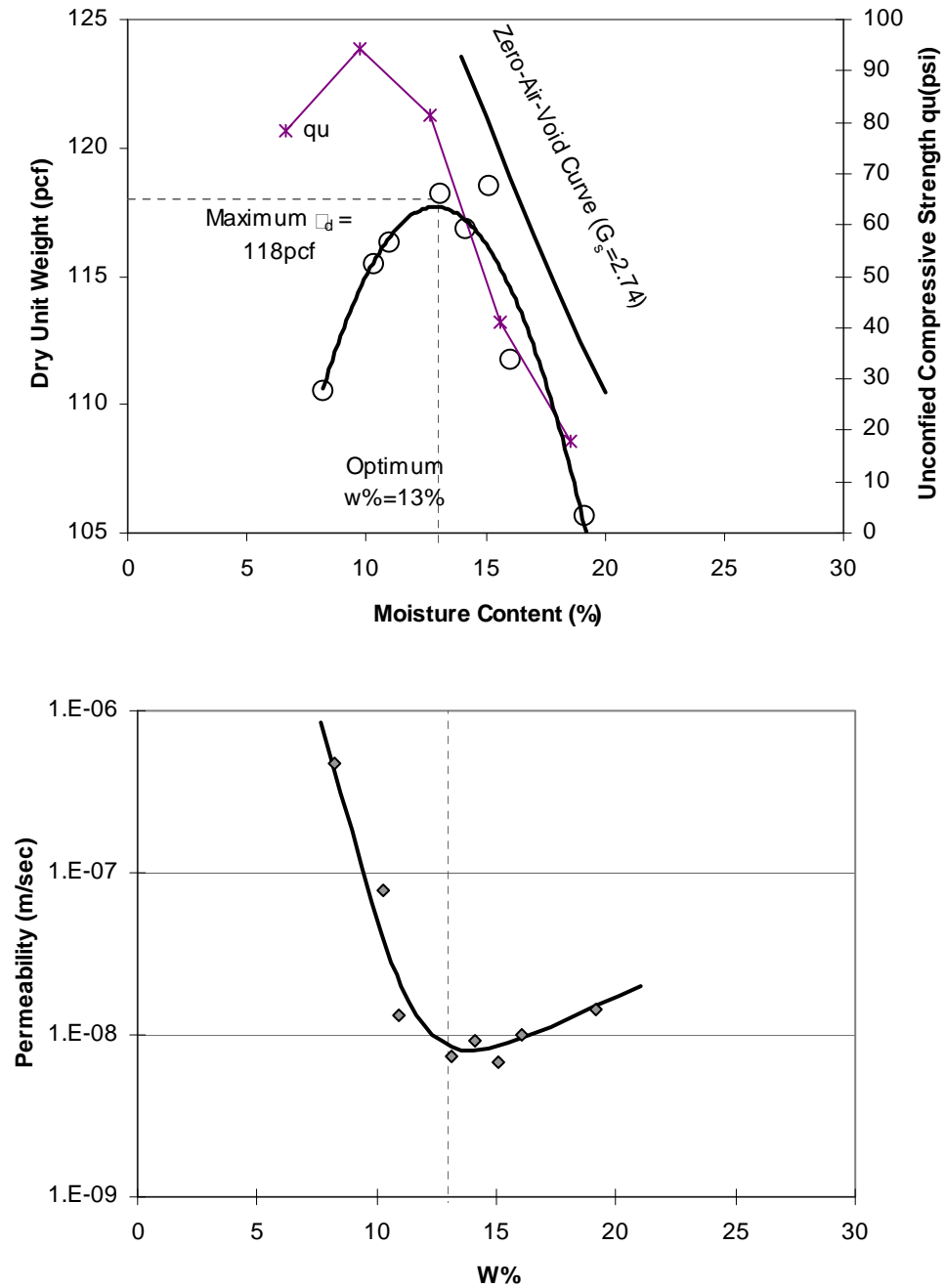
Figure 19. Compaction, permeability behavior of soil no. C
