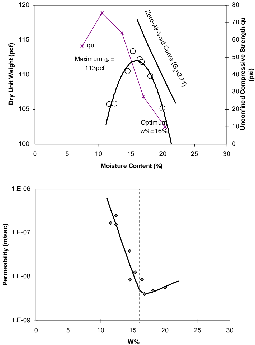
Figure 21. Compaction, permeability behavior of soil no. E
