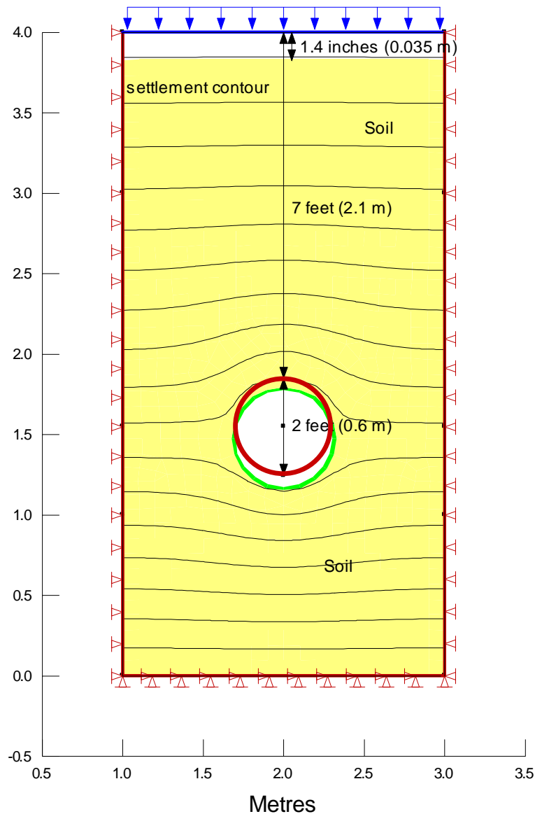
Figure 51(a). Settlement contour of pipe buried in soil (2 m wide trench)
