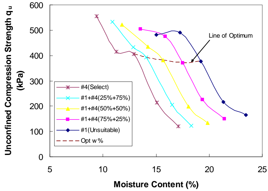
Figure 14(a). UCS of no. 4 and no. 1 blends
