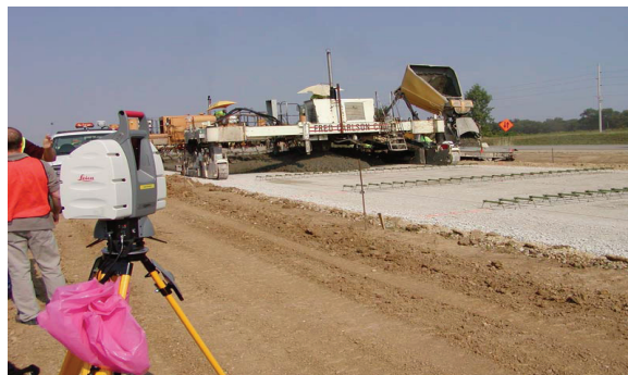
Performing laser scan on the subbase level
