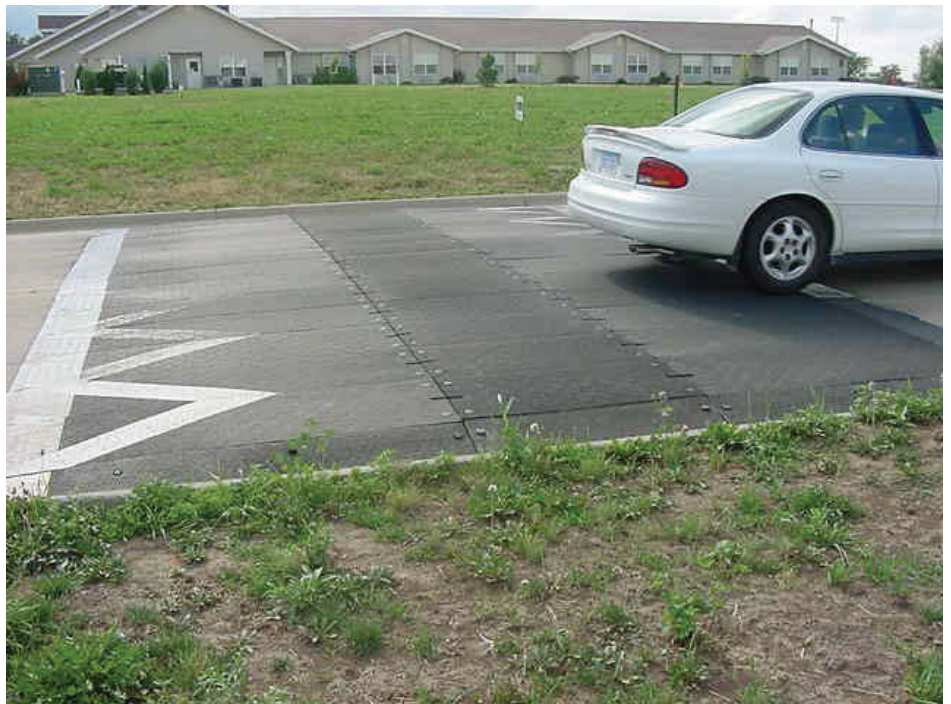
An example of a 30 mph speed table used in CTRE study for residential traffic calming in small Iowa communities.
